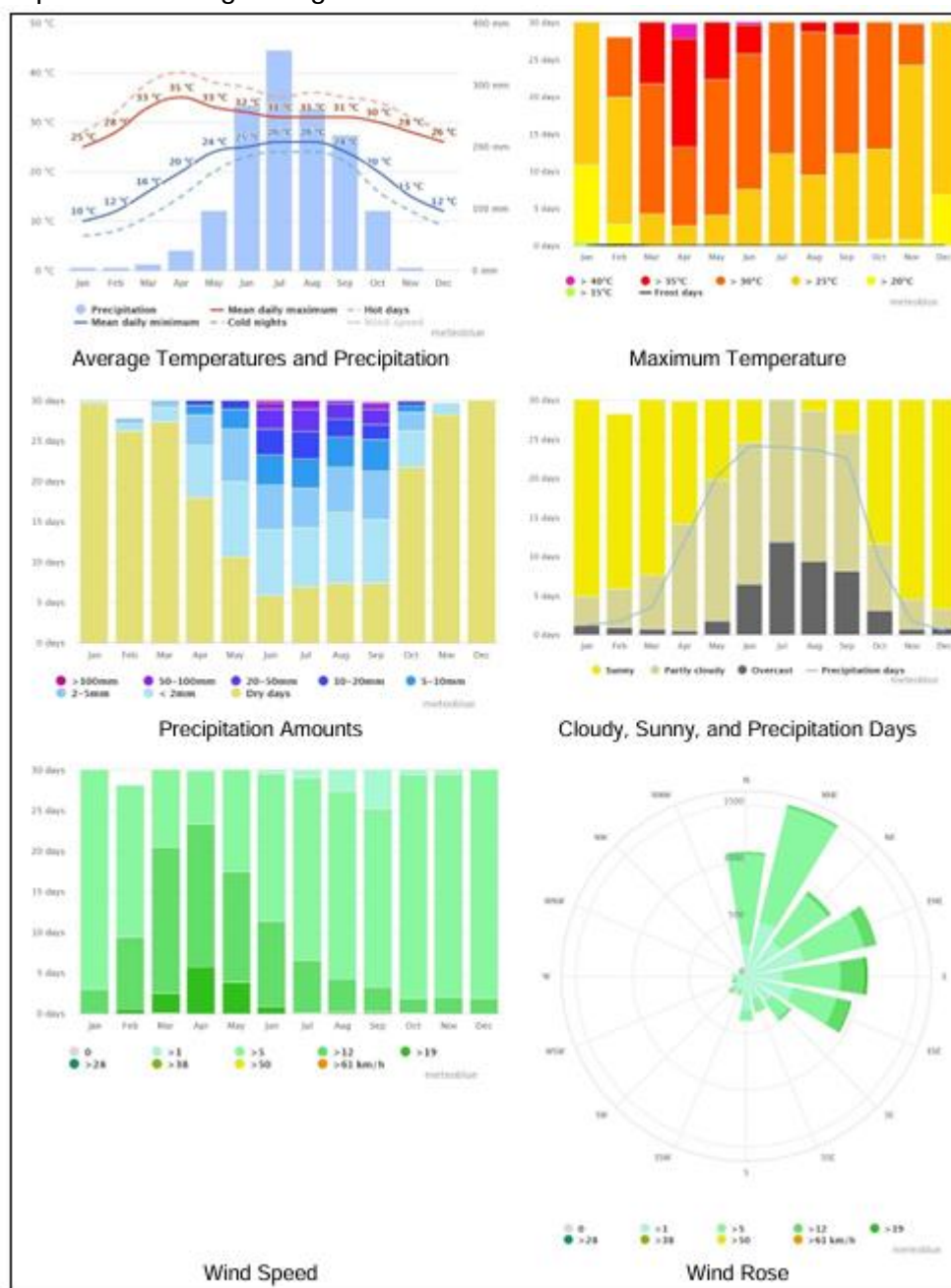
Figure 7: Historical Climatic Record at Patgram Region
