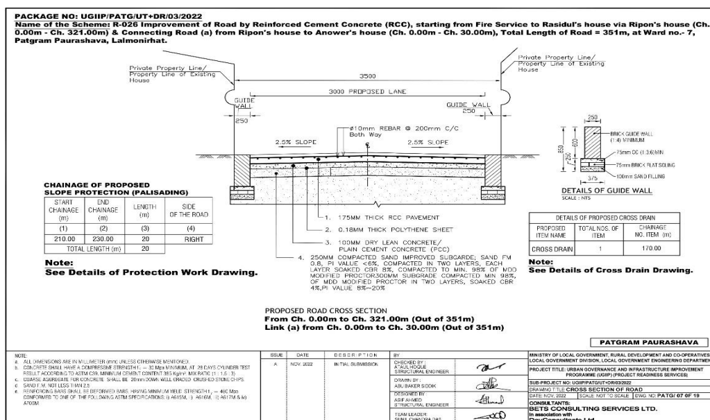
Figure 5: Cross-Section of Road in Pourashava
