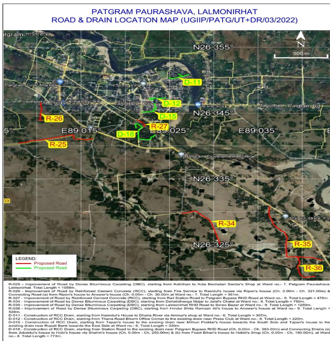
Figure 2: Google Earth of Proposed Roads & Drains in the Pourashava
