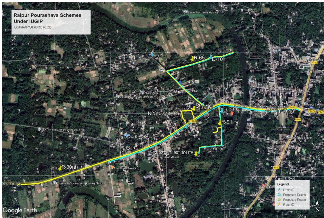
Figure III-5: Location of Roads and Drains at Raipur Pourashava
