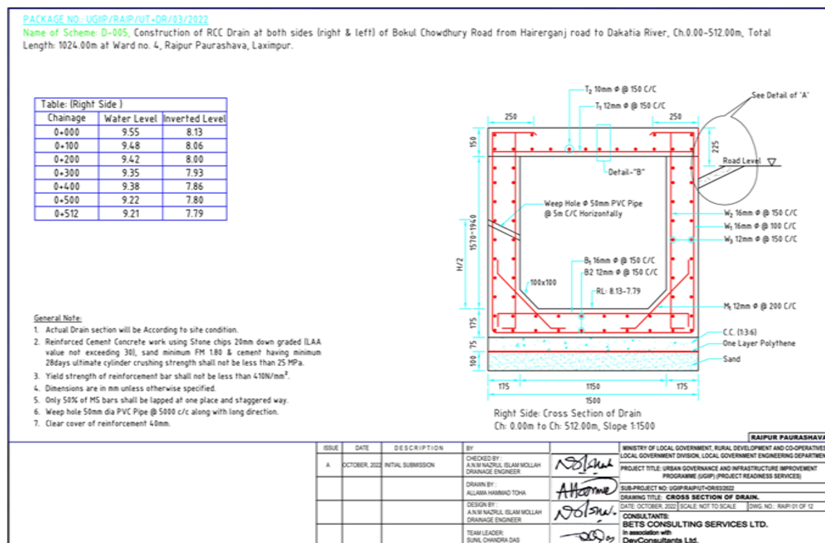
Figure 4: Cross-Section of Drain in Pourashava
