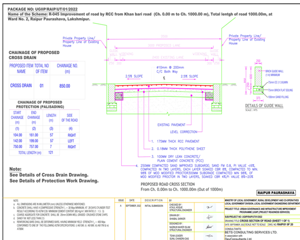
Figure 3: Cross-Section of Road in Pourashava
