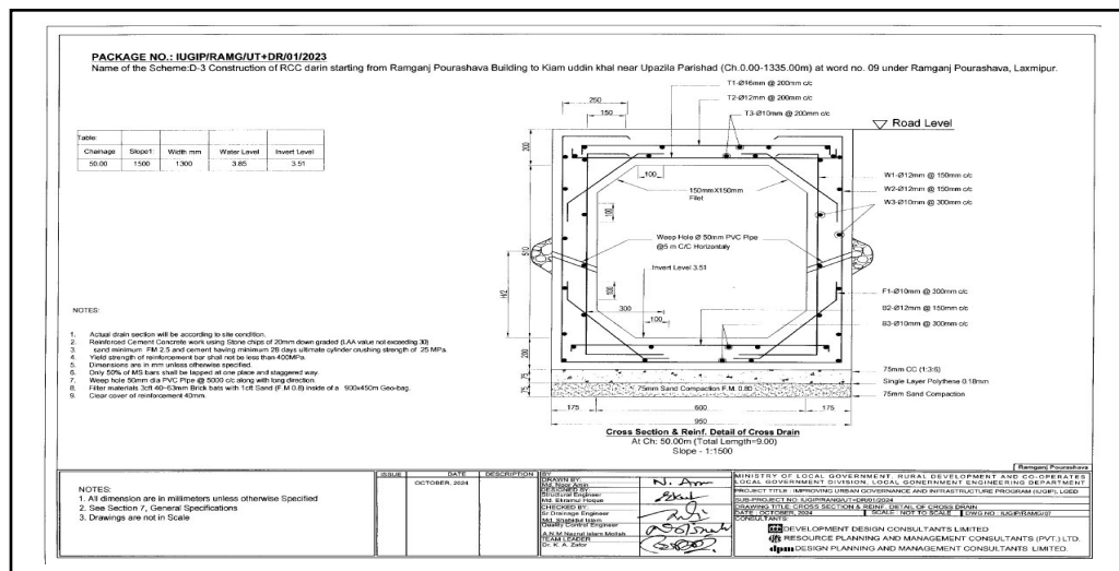
Figure III-4: Cross Section of Drain in Ramgani Pourashava
