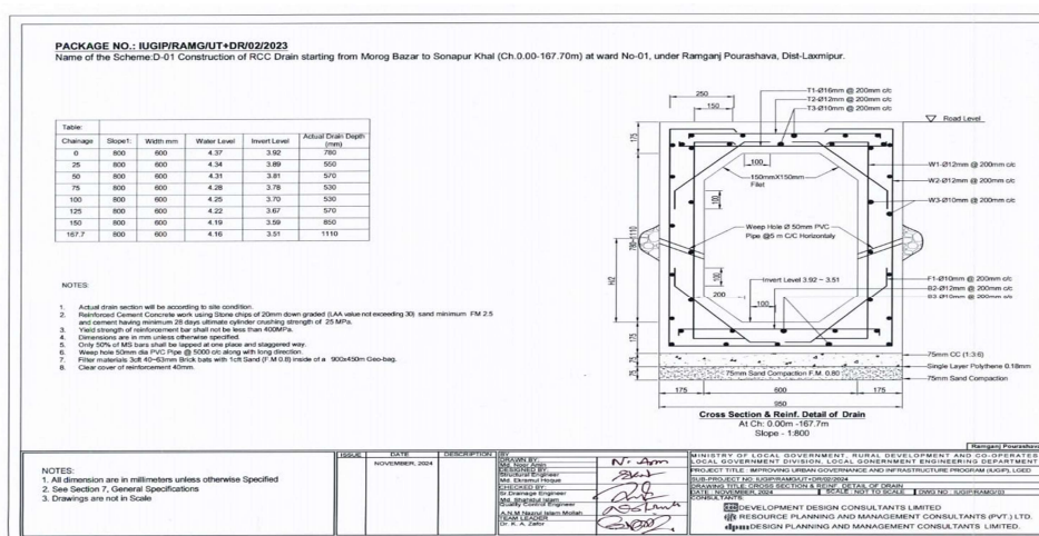
Figure III-4: Cross Section of Drain in Ramganj Pourashava
