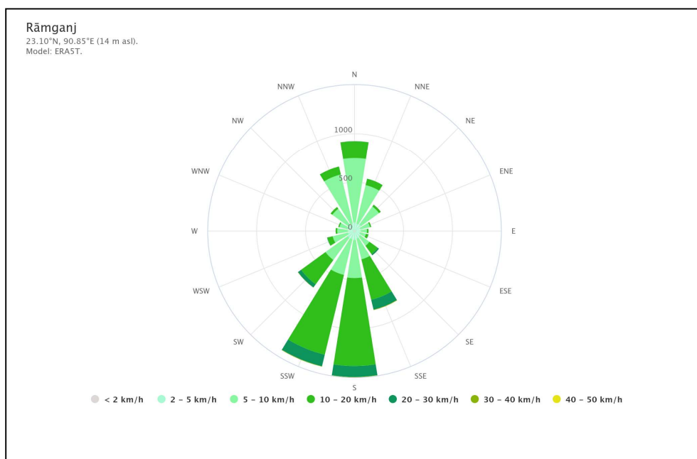
Figure IV-4: Wind Rose*
