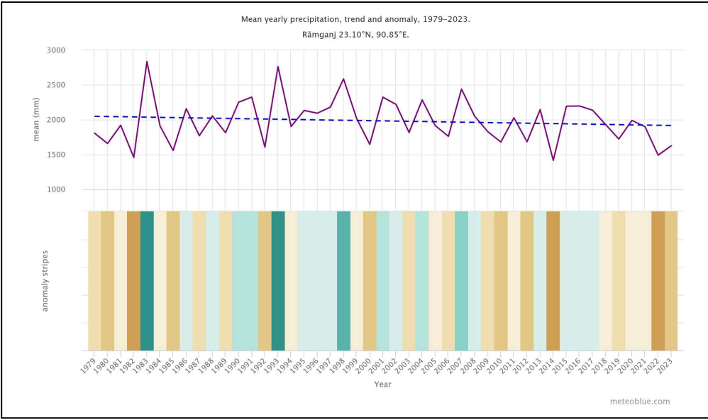
Figure IV-2: Yearly Precipitation Change*
