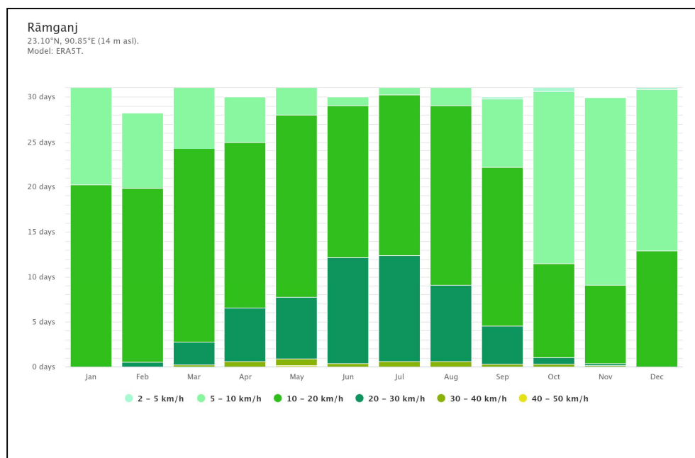
Figure IV-3: Wind Speed*
