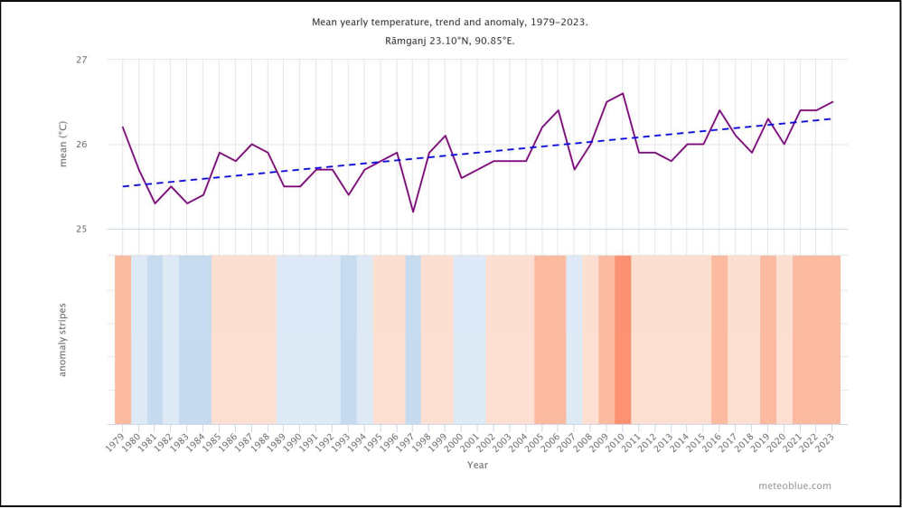
Figure IV-1: Yearly Temperature Change*
