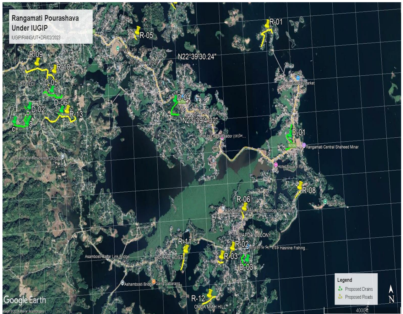
Figure III-5: Location of Roads, Drains at Rangamati Pourashava
