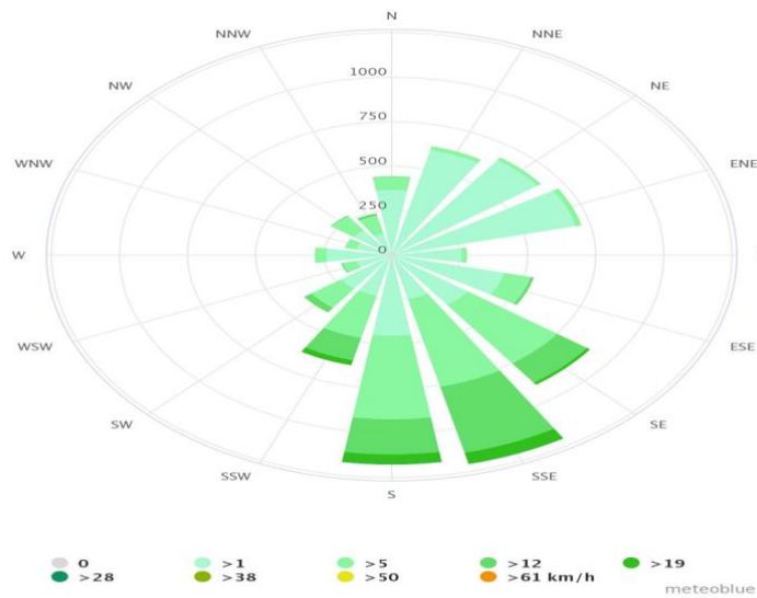
Figure IV-IV: Wind Rose*
