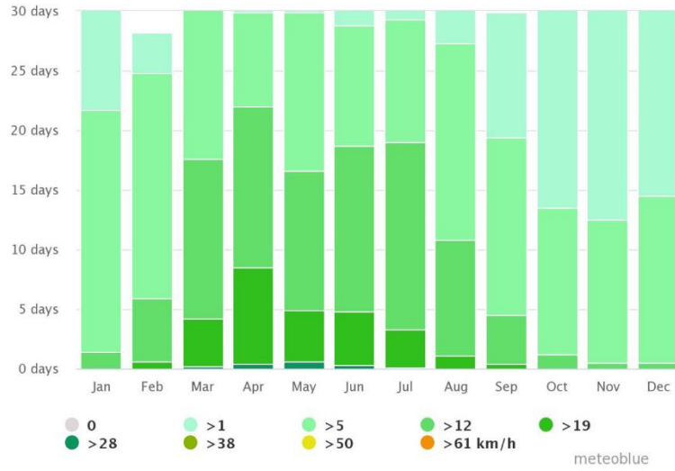
Figure IV-III: Wind Speed*
