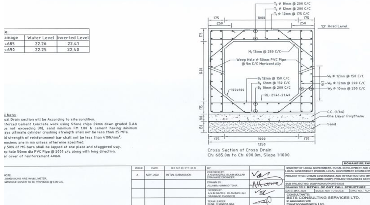
Figure 4: Cross-section of Drain Rohanpur Paurashava
