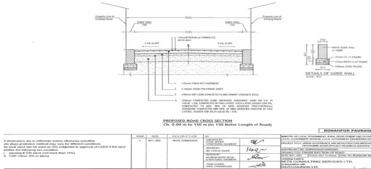
Figure 3: Cross-Section of Road Rohanpur Paurashava
