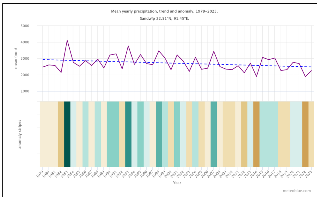
Figure IV-II: Yearly Precipitation Change*
