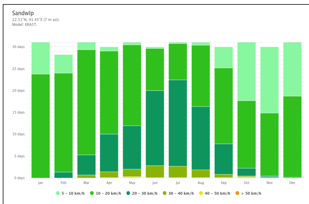
Figure IV-III: Wind Speed*
