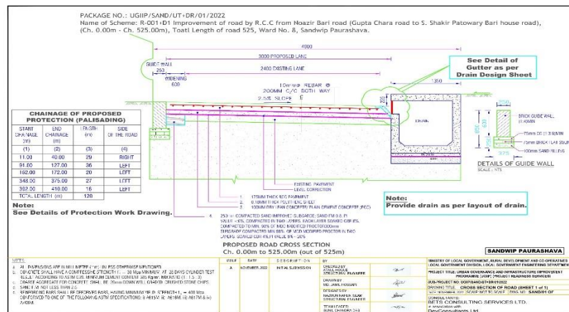
Figure III-III: Cross Section of Road in Sandwip Pourashava
