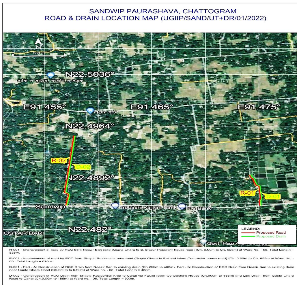
Figure III-V: Location of Roads, Drain at Sandwip Pourashava
