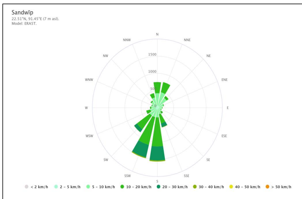
Figure IV-IV: Wind Rose*
