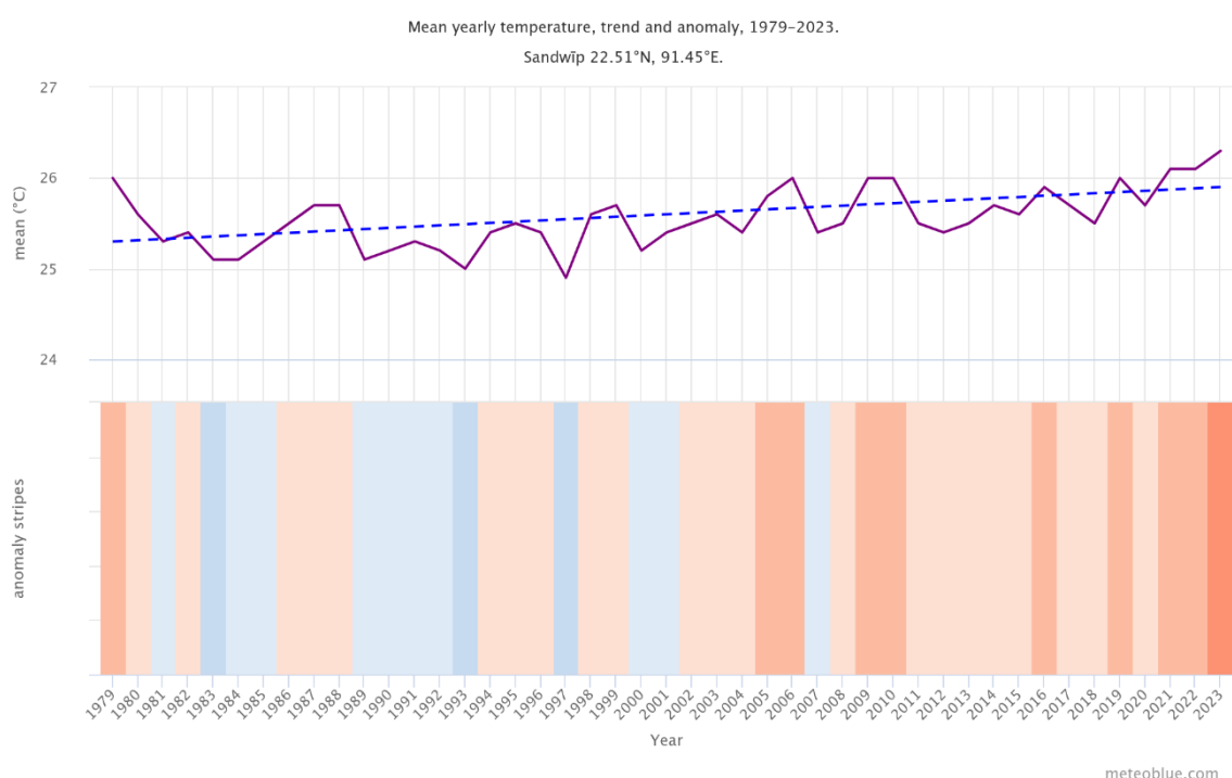
Figure IV-I: Yearly Temperature Change*
