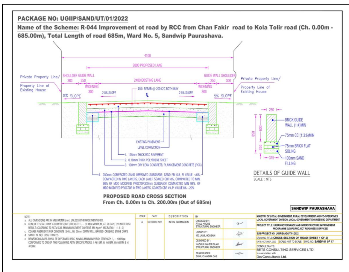
Figure III-III: Cross Section of Road in Sandwip Pourashava
