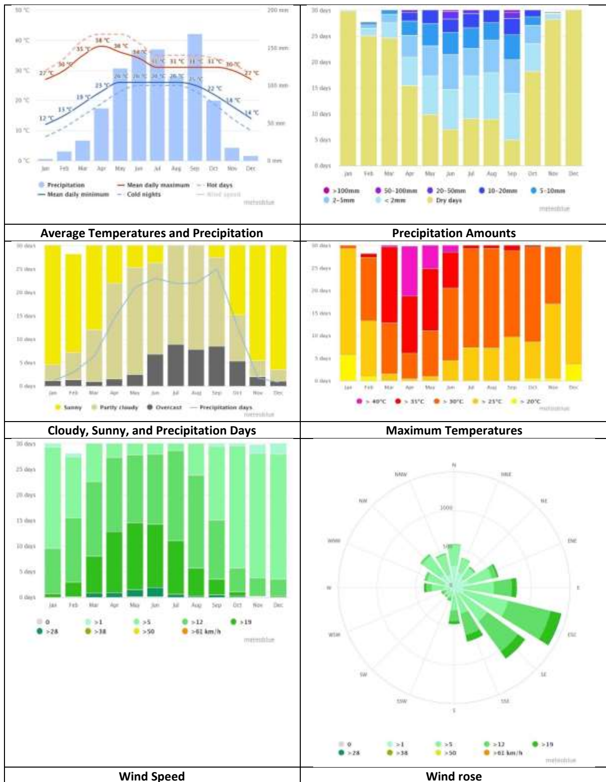
Figure 7: Historical Climatic Record at Santhia Region
