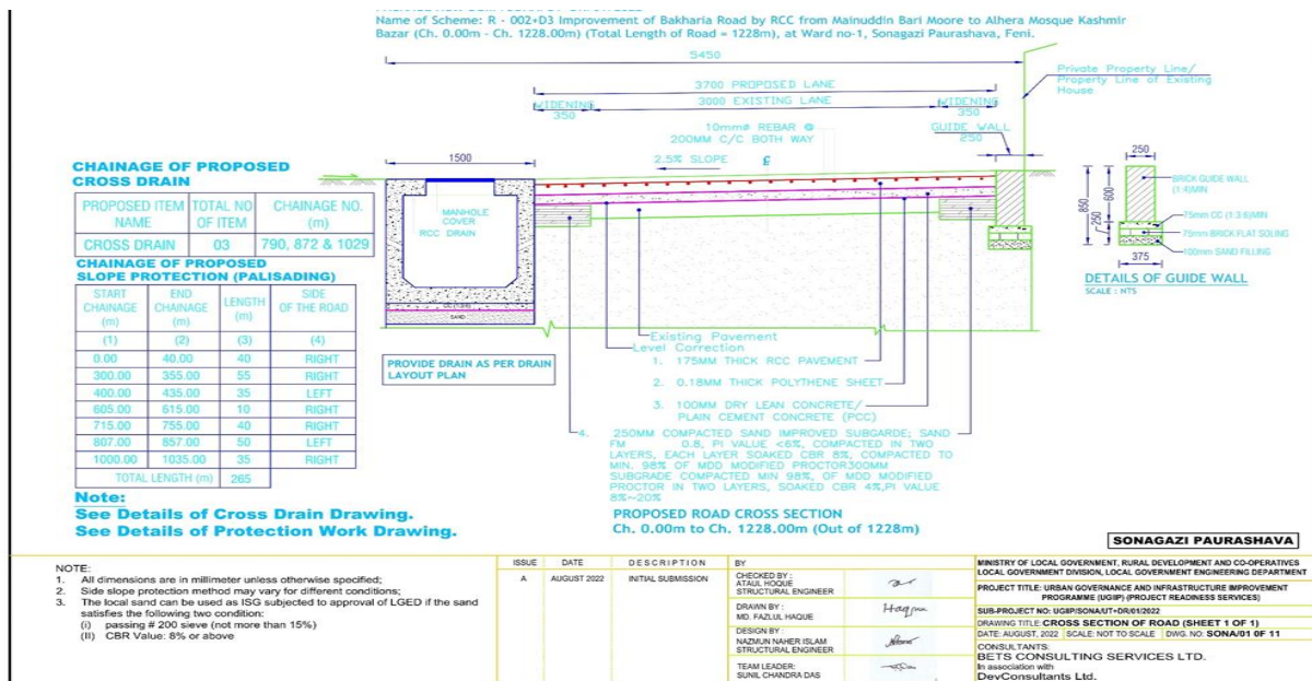
Figure 4: Cross-Section of Drain in Pourashava
