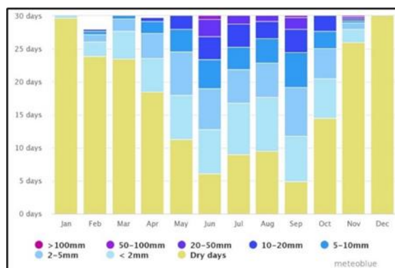
Precipitation Amounts
