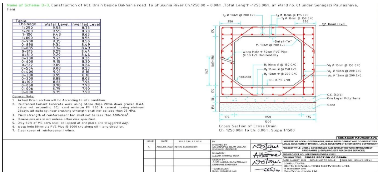
Figure 5: Cross-Section of Drain in Pourashava
