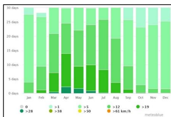
Wind Speed
