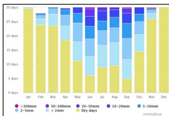
Precipitation Amounts
