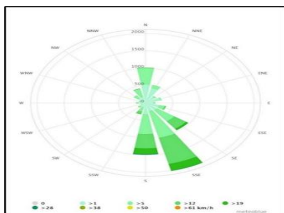
Wind Rose
