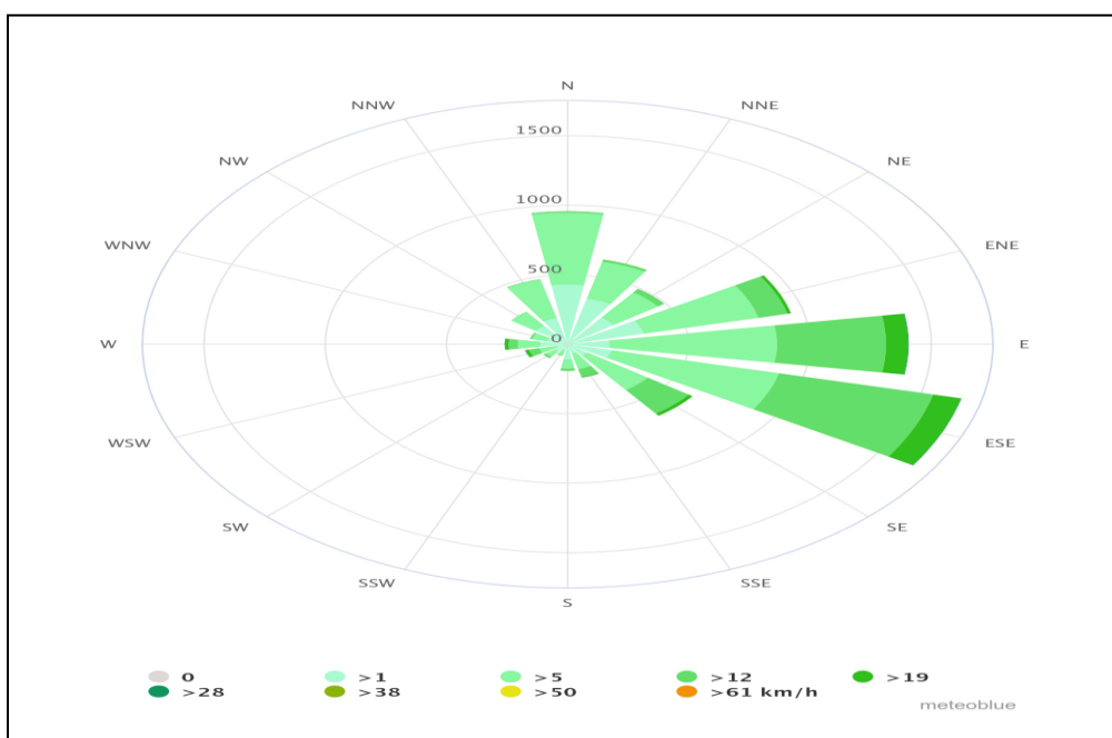
Figure IV-4: Wind Rose*
