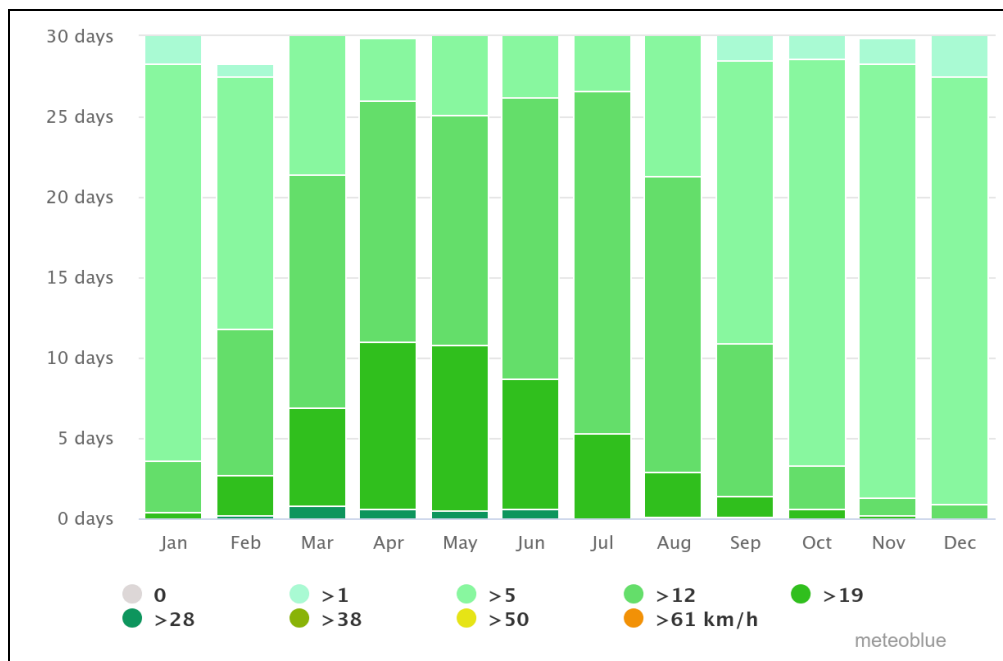
Figure IV-3: Wind Speed*
