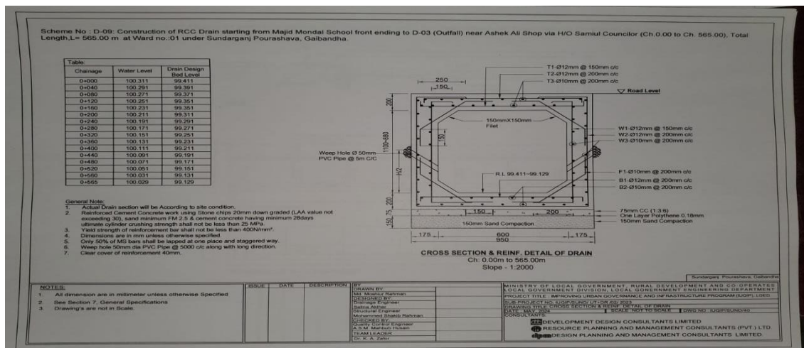
Figure III-4: Cross Section of Drain in Sundarganj Pourashava
