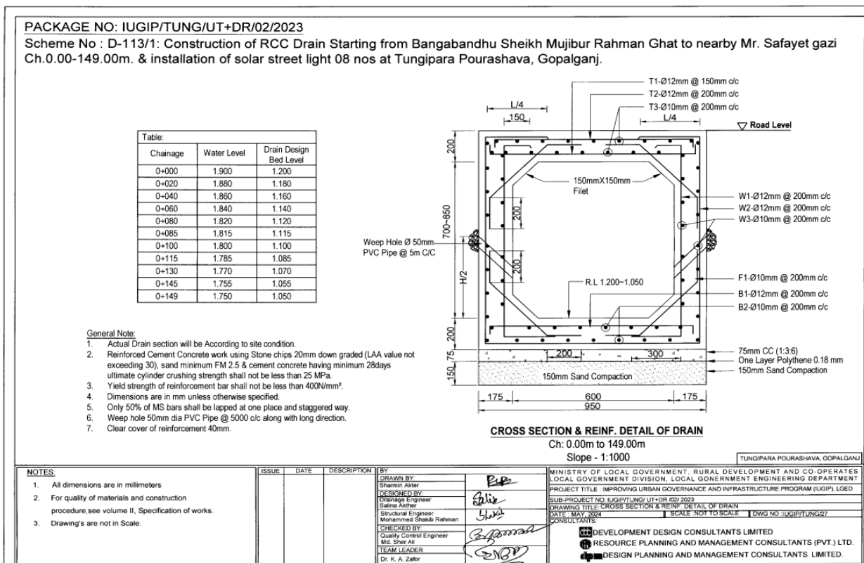
Figure 4: Cross-Section of Drain in Pourashava
