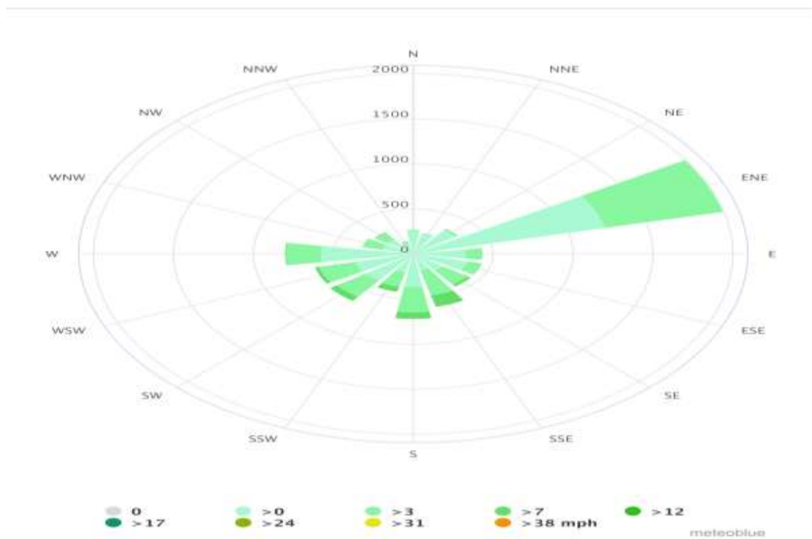
Figure IV-4: Wind Rose*
