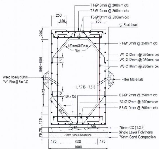
Cross Section & Reinf. Detail of Drain Ch: 0.00m to Ch:220.00m, Total Length=220m Slope-1:1000
