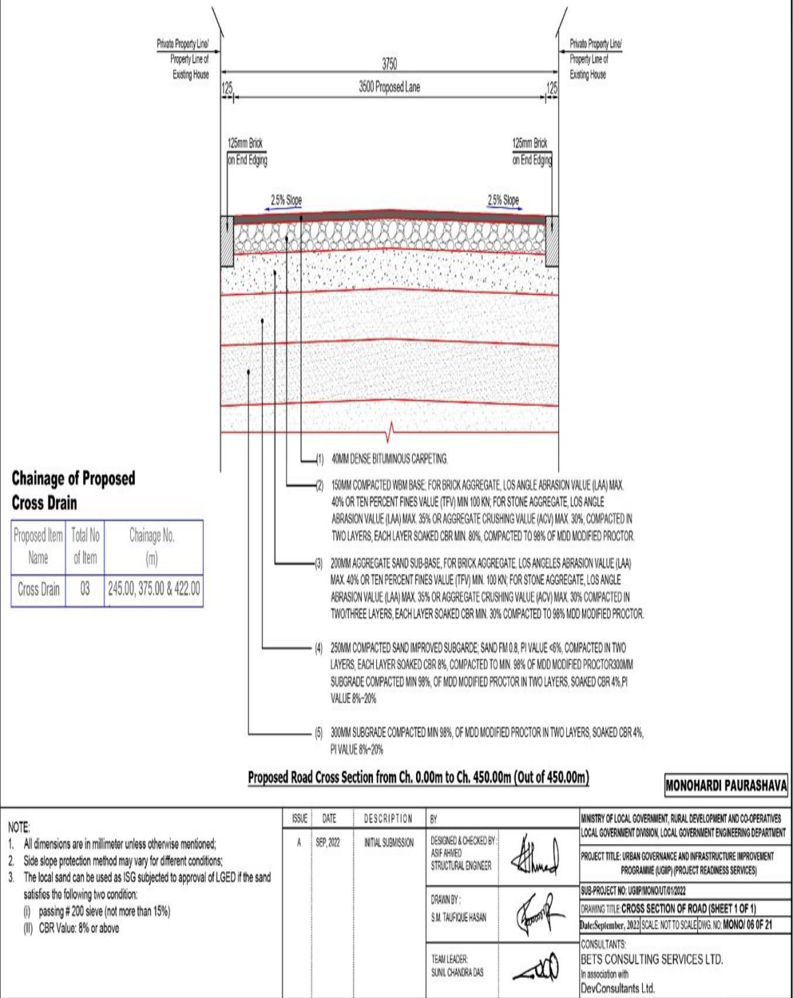
Figure 3: Cross-Section of Road in Pourashava
