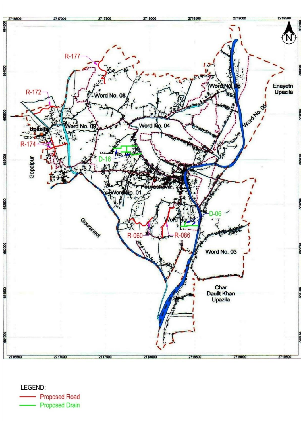
Figure- 3: Road layout of the proposed subproject
