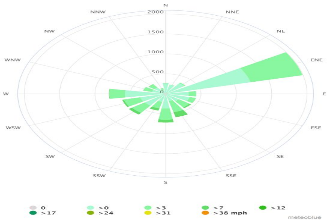
Figure IV-4: Wind Rose*
