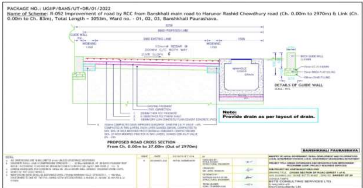
Figure 3: Cross-Section of Road in Banskhal Paurashava
