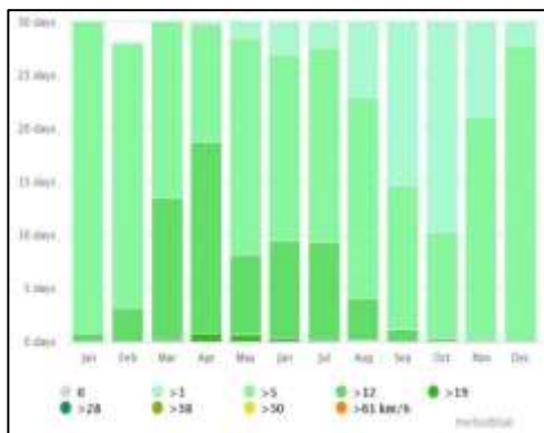
Wind Speed
