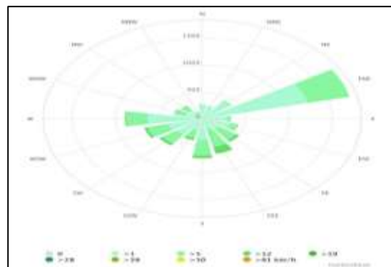
Wind Rose
