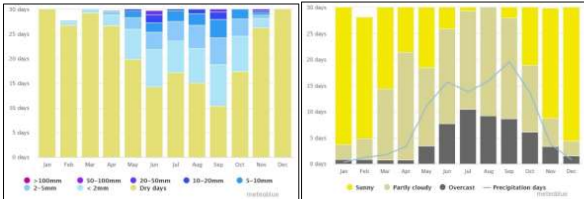
Precipitation Amounts
