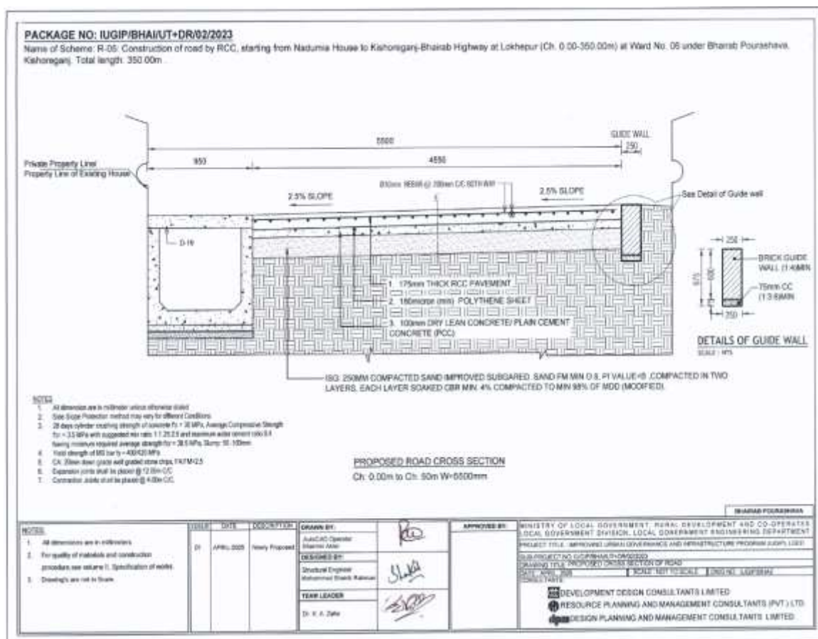
Figure III-3: Cross Section of Road in Bhairab Pourashava
