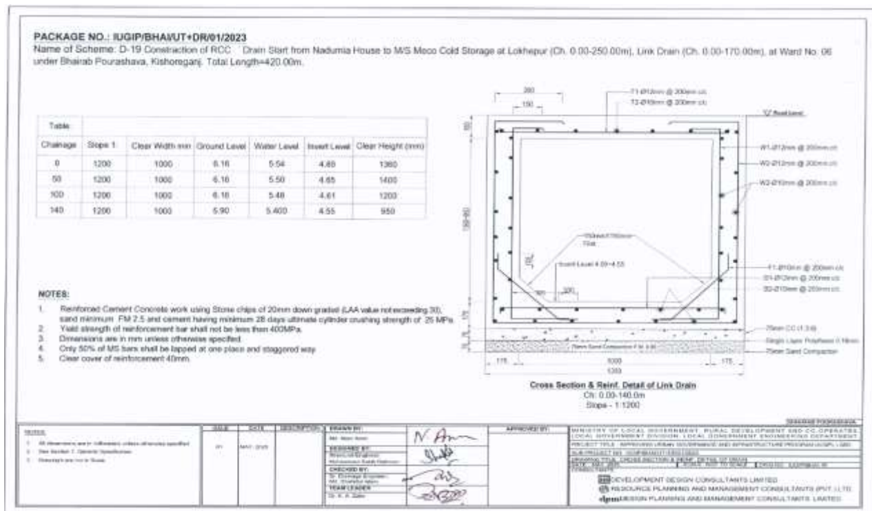
Figure III-4: Cross Section of Drain in Bhairab Pourashava
