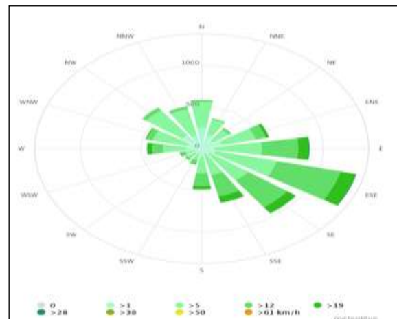
Wind rose
