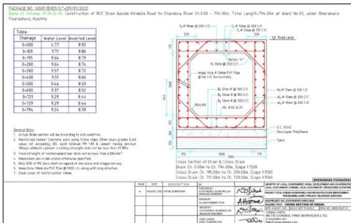
Figure 5: Cross-Section of Drain in the Bheramara Pourashava
