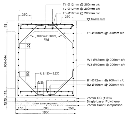
Cross Section & Reinf. Detail of Drain Ch: 0.00m to Ch:200.00m, Total Length=200.00m Slope=1:1000
