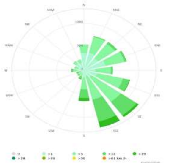
Wind Rose
