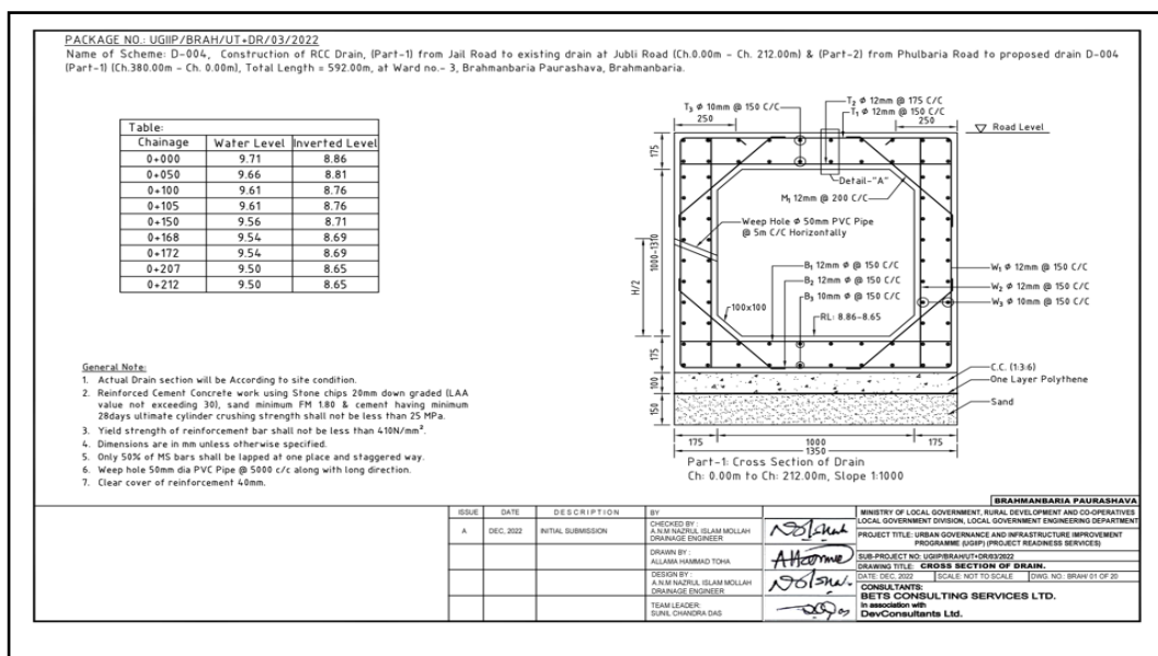
Figure III-4: Cross Section of Drain in Brahmanbaria Pourashava
