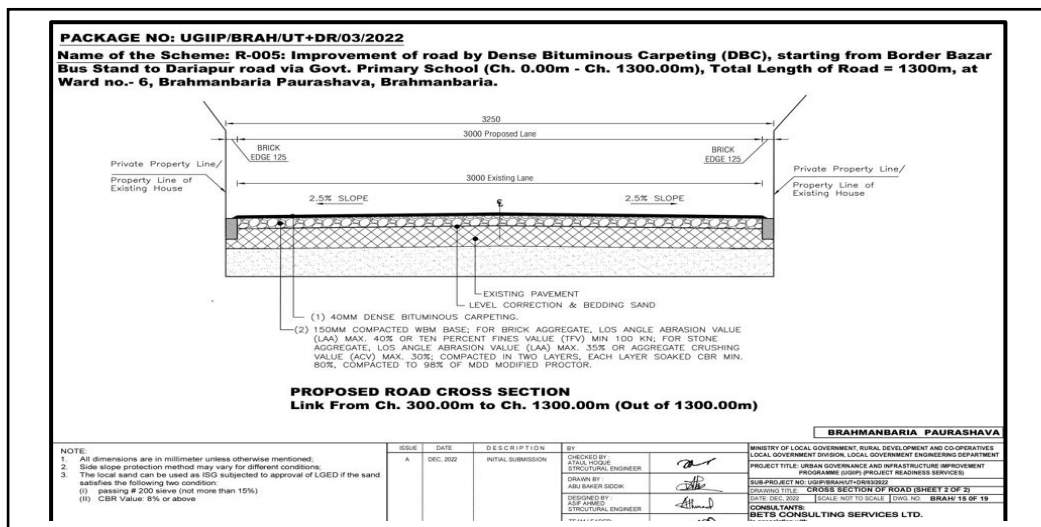
Figure III-3: Cross Section of Road in Brahmanbaria Pourashava
