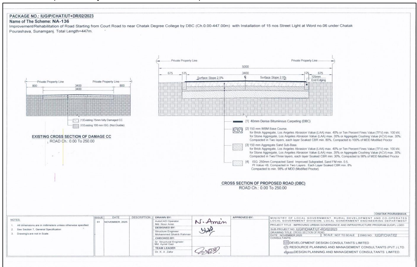
Figure III-3: Cross Section of Road in Chhatak Pourashava
