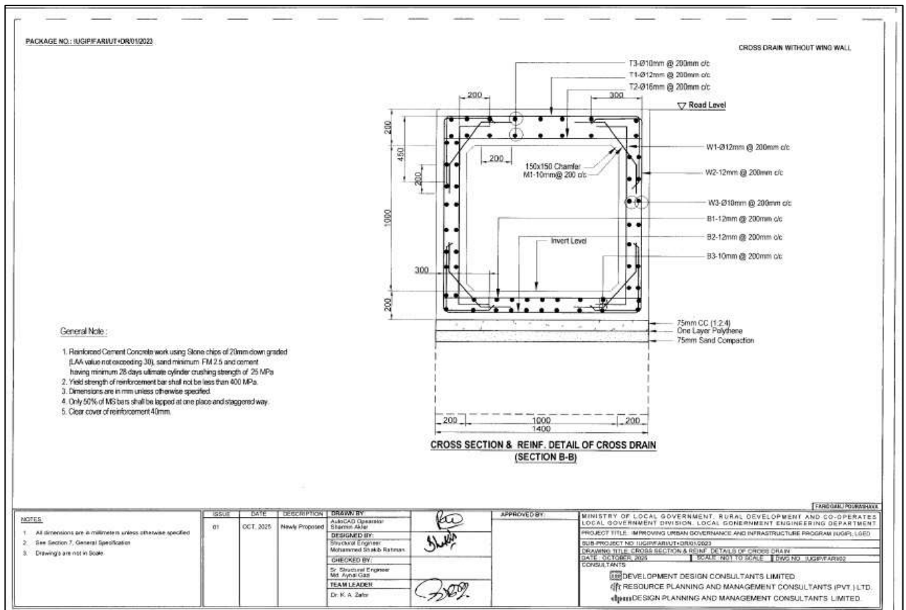
Figure 5: Cross-Section of Drain Faridganj Pourashava
