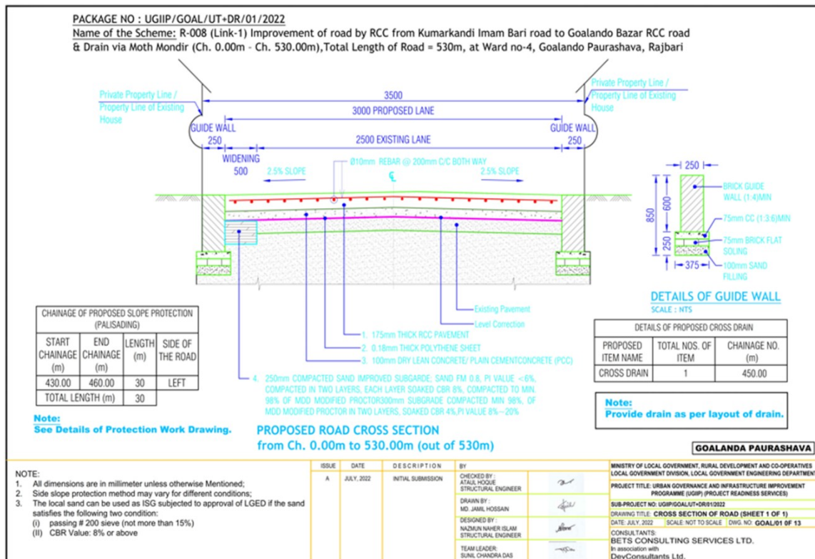
Figure 3: Cross-Section of Road in Goalando
