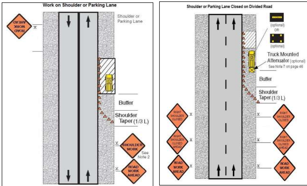
Figure A2 & A3: Work on shoulder or parking lane and shoulder or parking lane closed on divided road
