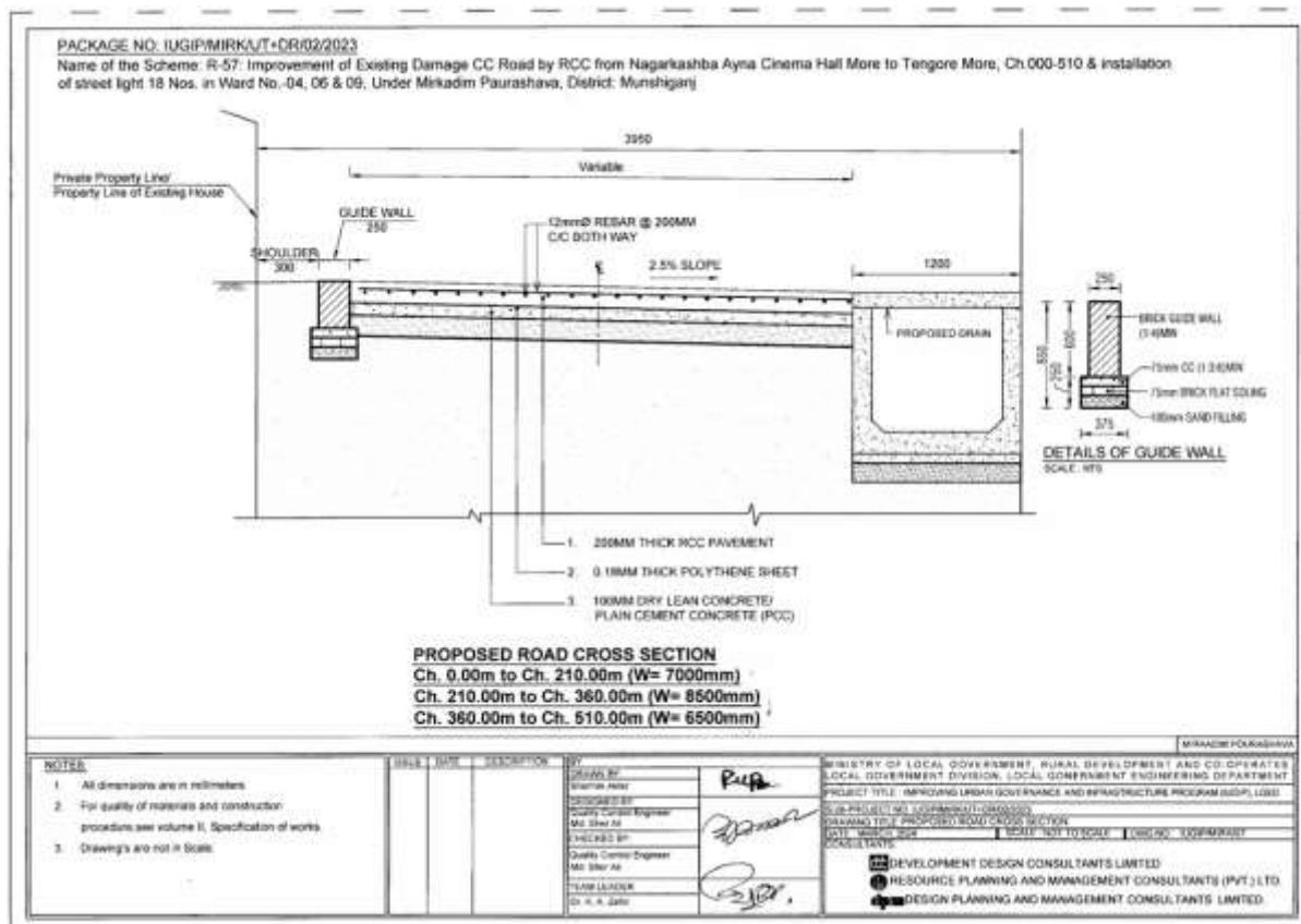
Figure 5: Cross-Section of Drain in Pourashava
