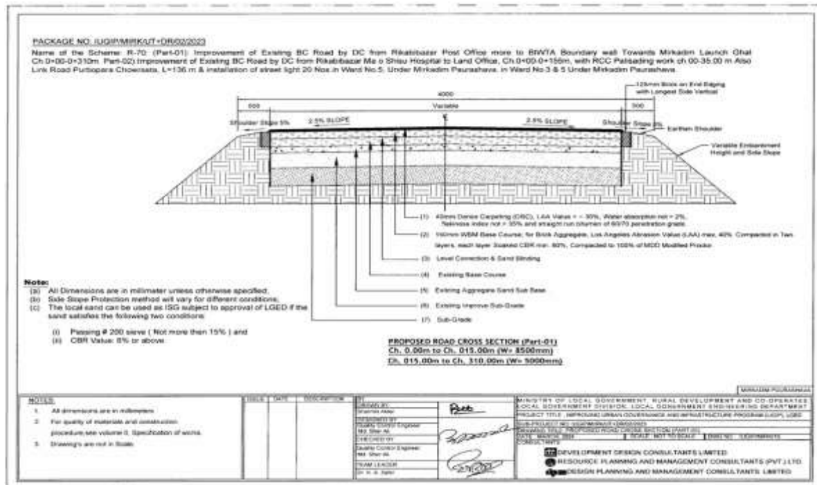
Figure 4: Cross-Section of Road in Pourashava
