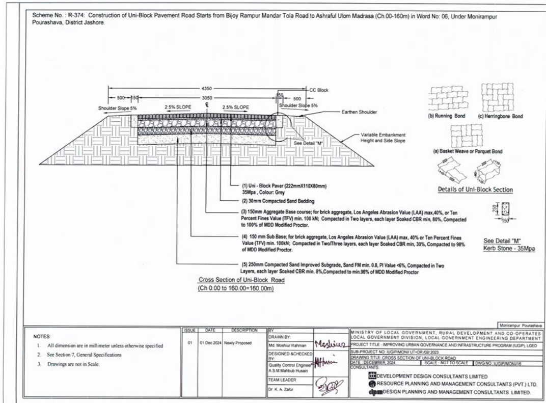
Figure 3: Cross-Section of Road in Monirampur Pourashava
