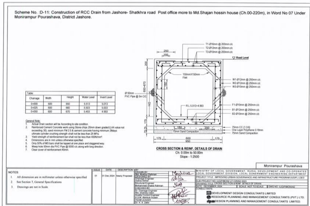
Figure 4: Cross-Section of Drain in Monirampur Pourashava
