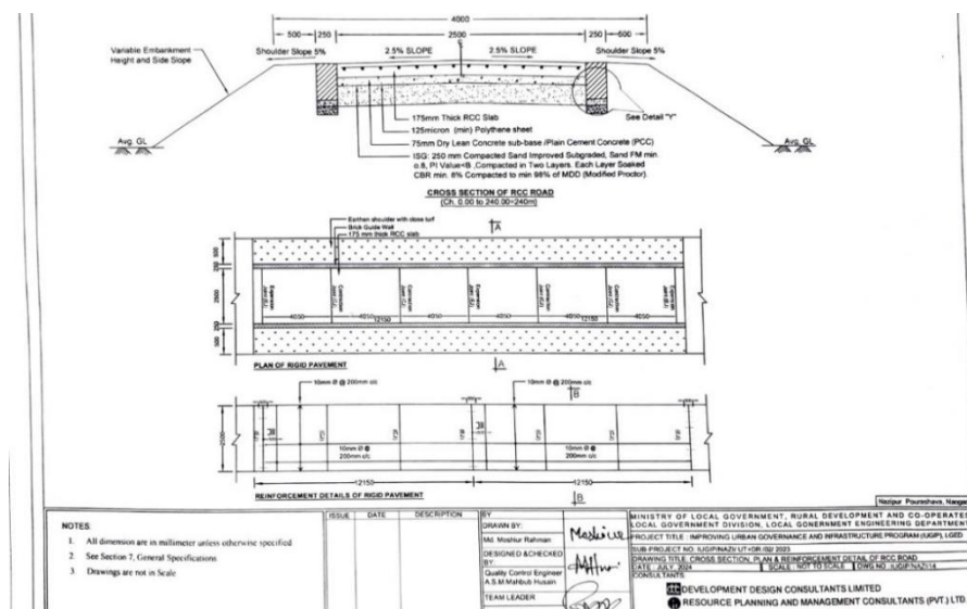
Figure 3: Cross-Section of Road in Pourashava
