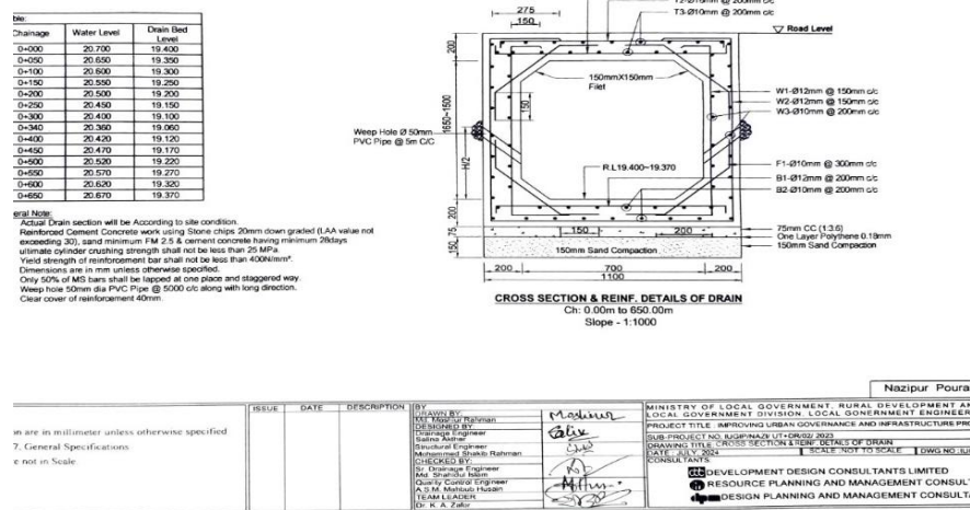
Figure 4: Cross-Section of Drain in Pourashava
