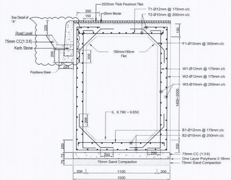
CROSS SECTION & REINF. DETAILS OF DRAIN (WITH KERB STONE) Ch: 0.00m to Ch:210.00m, Total Length=210m Slope - 1:1500
