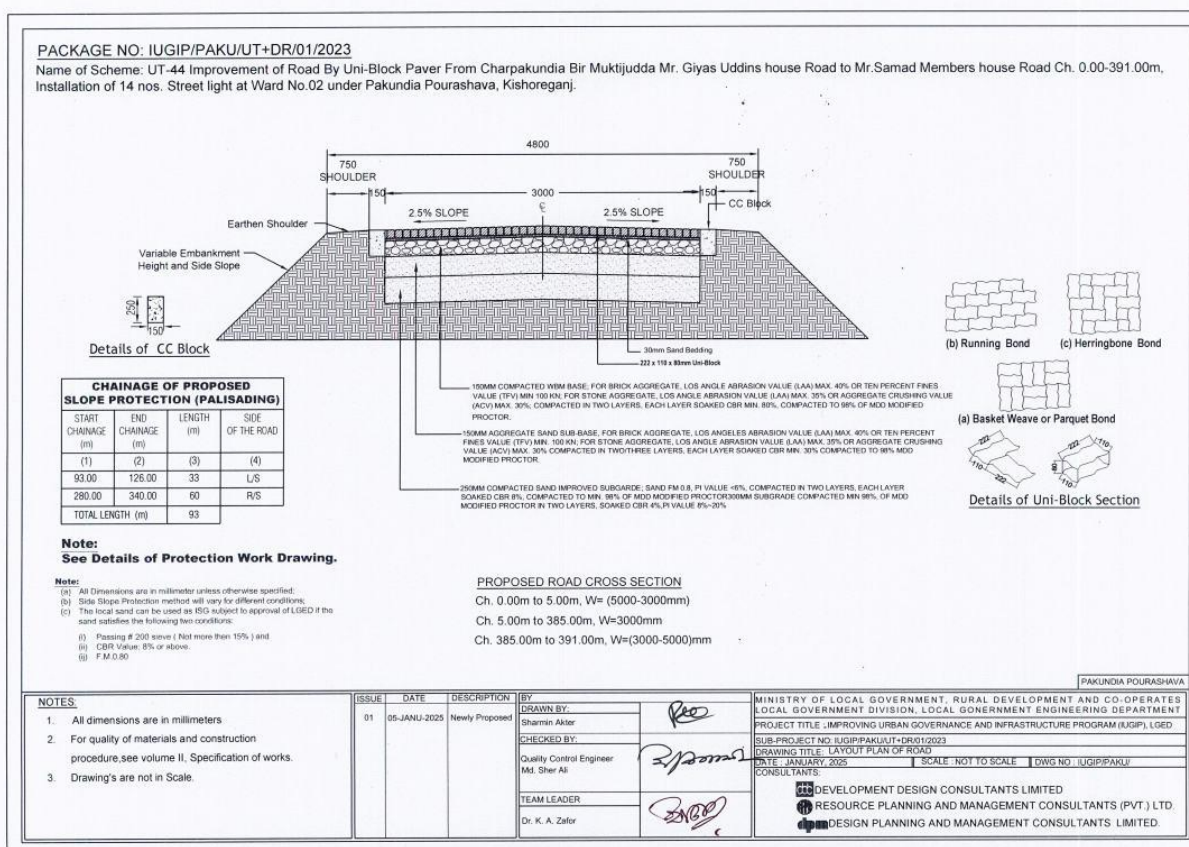
Figure 03: Cross-Section of Road in Pourashava
