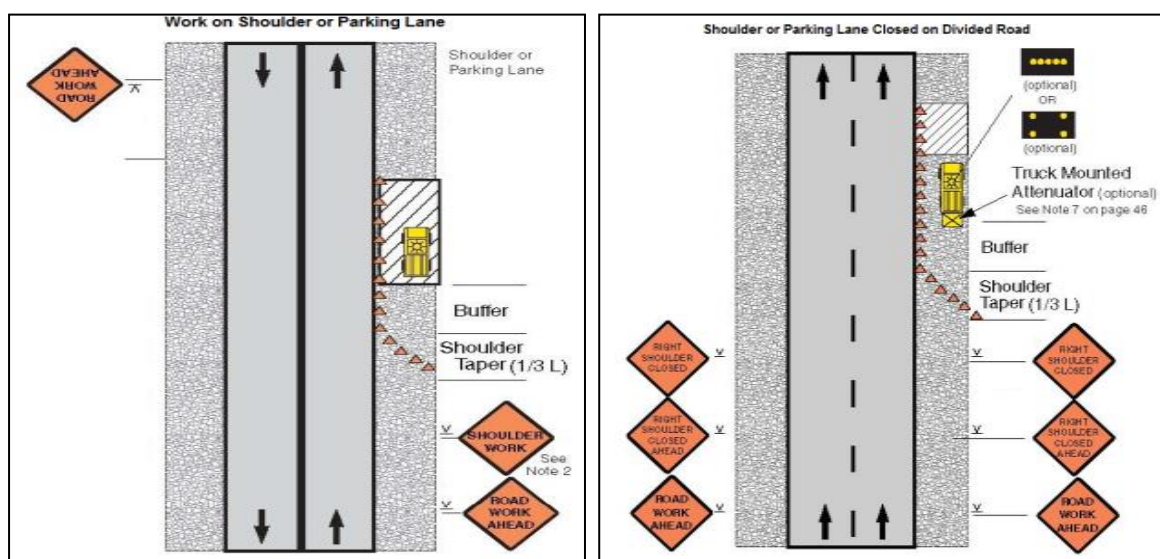
Figure A2 & A3: Work on shoulder or parking lane and shoulder or parking lane closed on
