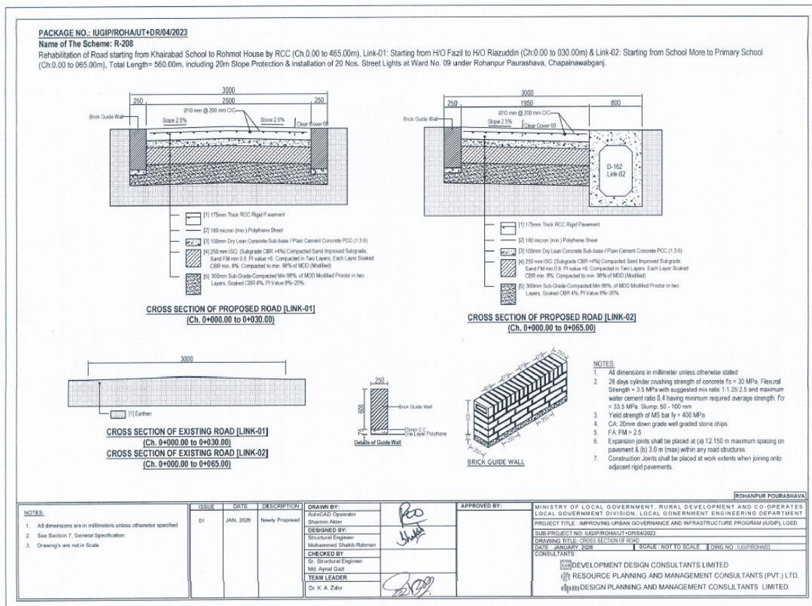
Figure 3: Cross-Section of Road Rohanpur Paurashava
