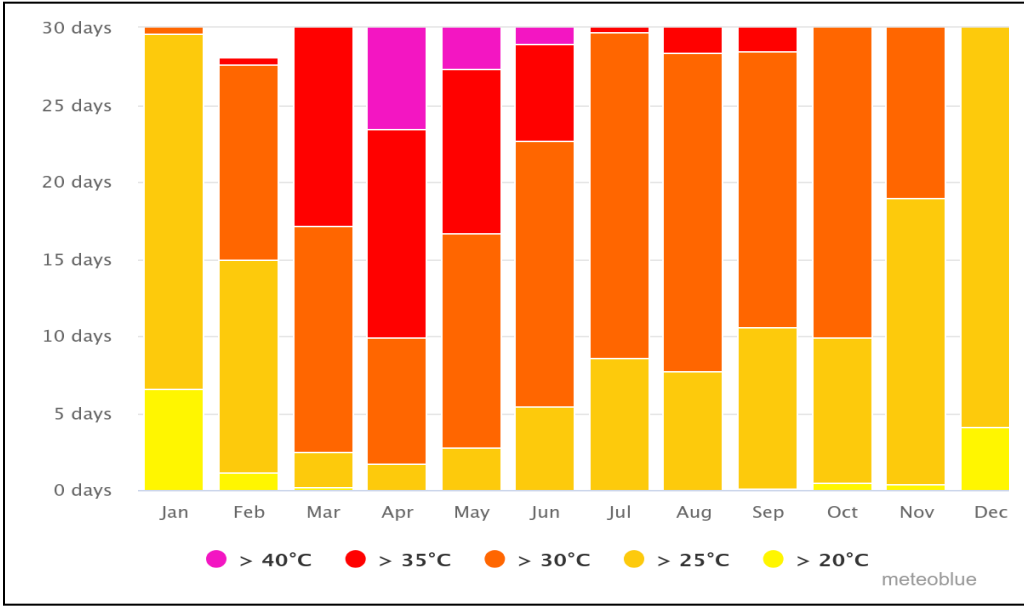
Figure IV-2: Maximum Temperature*
