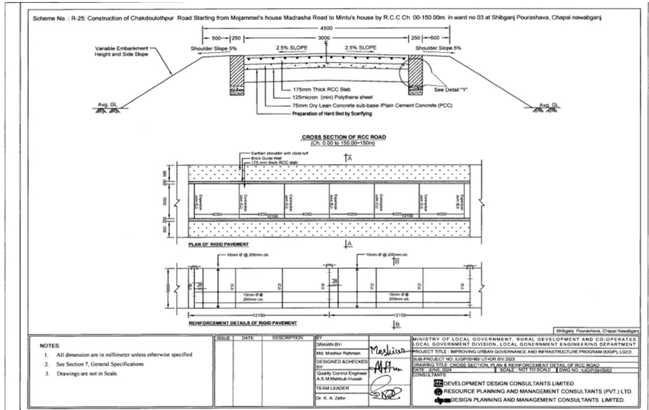
Figure 3: Cross-Section of Road in Pourashava
