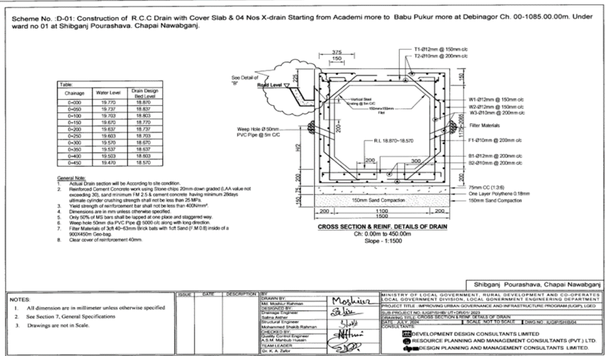
Figure 4: Cross-Section of Drain in Pourashava
