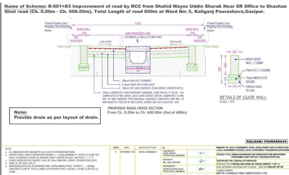
Figure III-4: Cross Section of Road in Kaliganj Pourashava
