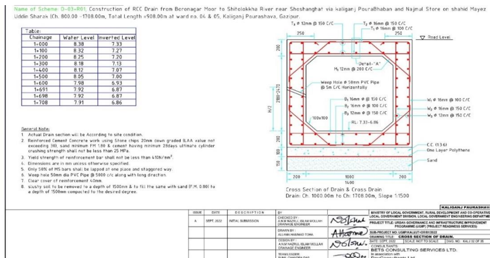
Figure III-5: Cross Section of Drain in Kaliganj Pourashava
